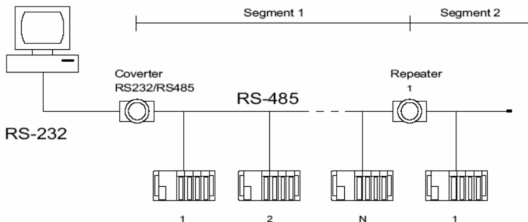
Figure C-1: Daisychaining
