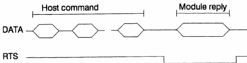
Figure C-6: RS-485 data flow control with RTS
