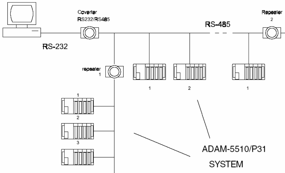
Figure C-3: Random structure
