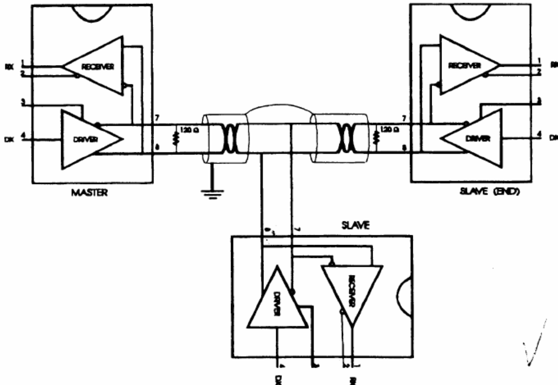
Figure C-5: Termination resistor locations
