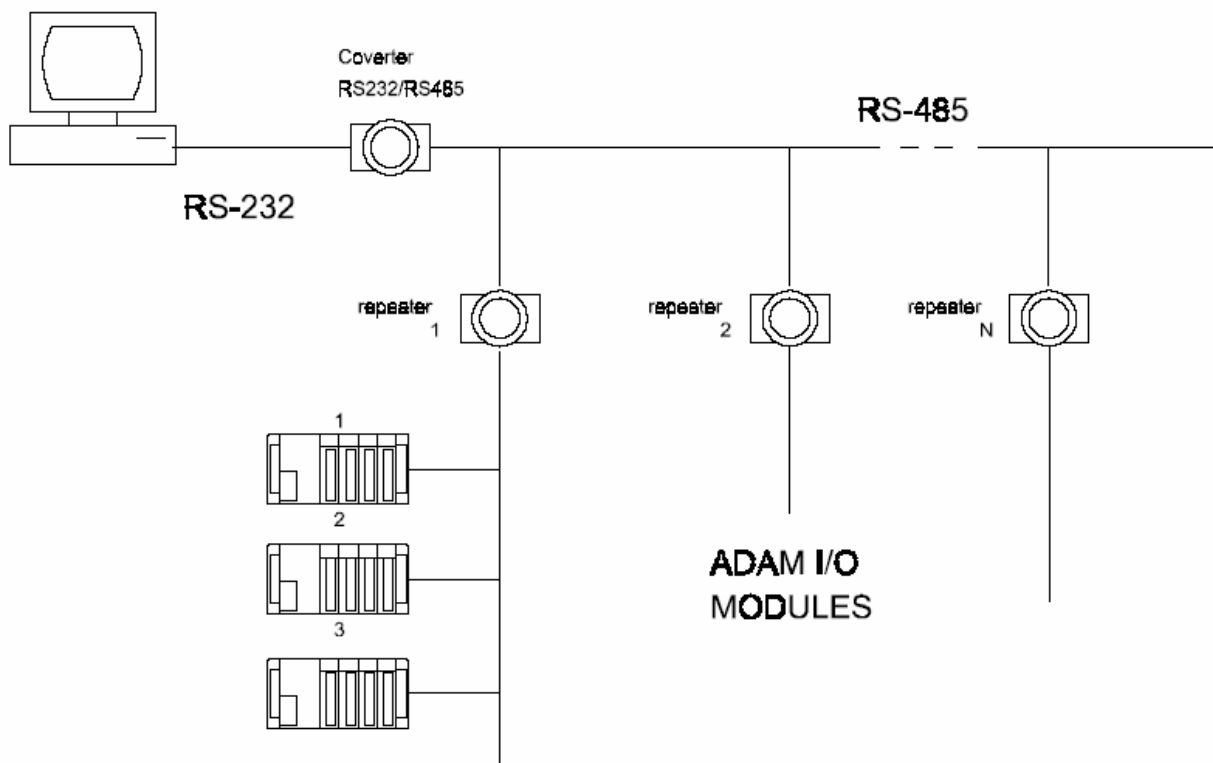
Figure C-2: Star structure
