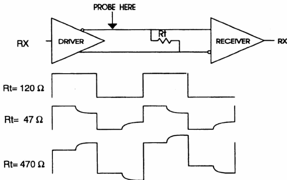
Figure C-4: Signal distortion
